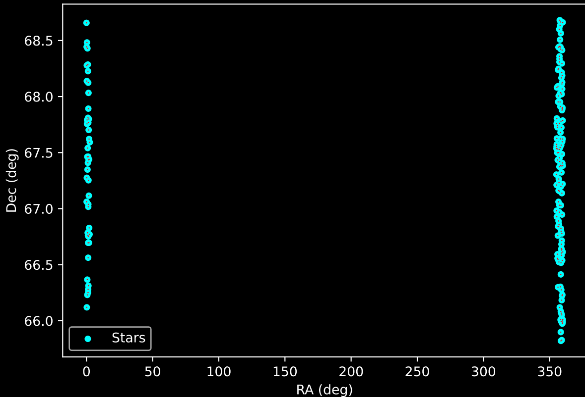
APOGEE DR17 Field: [CVZTILE_098+34_btx] Proper Motion Vectors for Gaia Star Field ( n = 176 )
