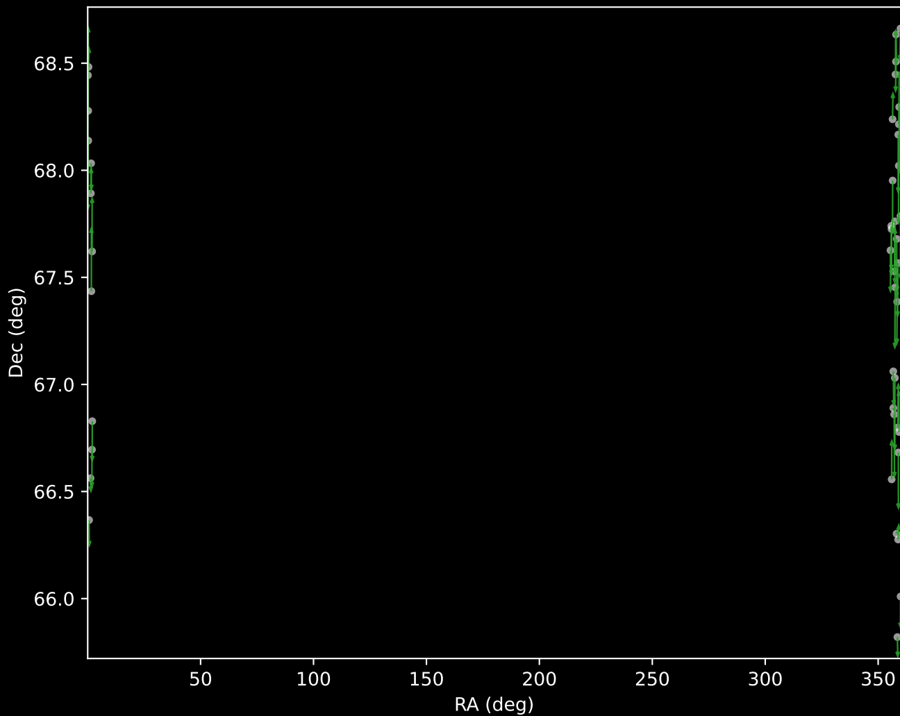
APOGEE DR17 Cluster 4 Proper Motion Vectors (n=44)
