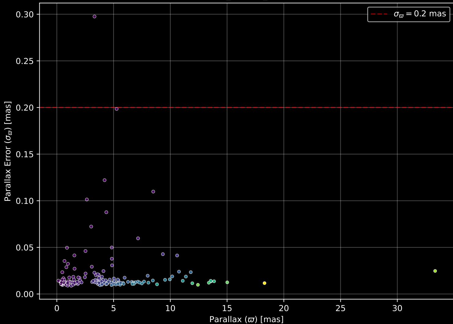
APOGEE DR17 Field: [CVZTILE_098+34_btx] Parallax Quality (n= 176)
