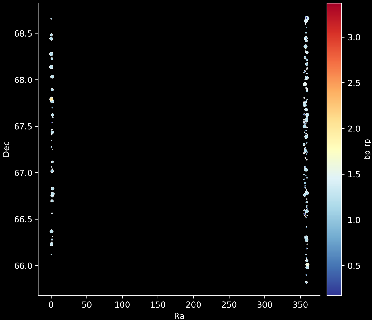
APOGEE DR17 Field: [CVZTILE_098+34_btx] Stars: 176
