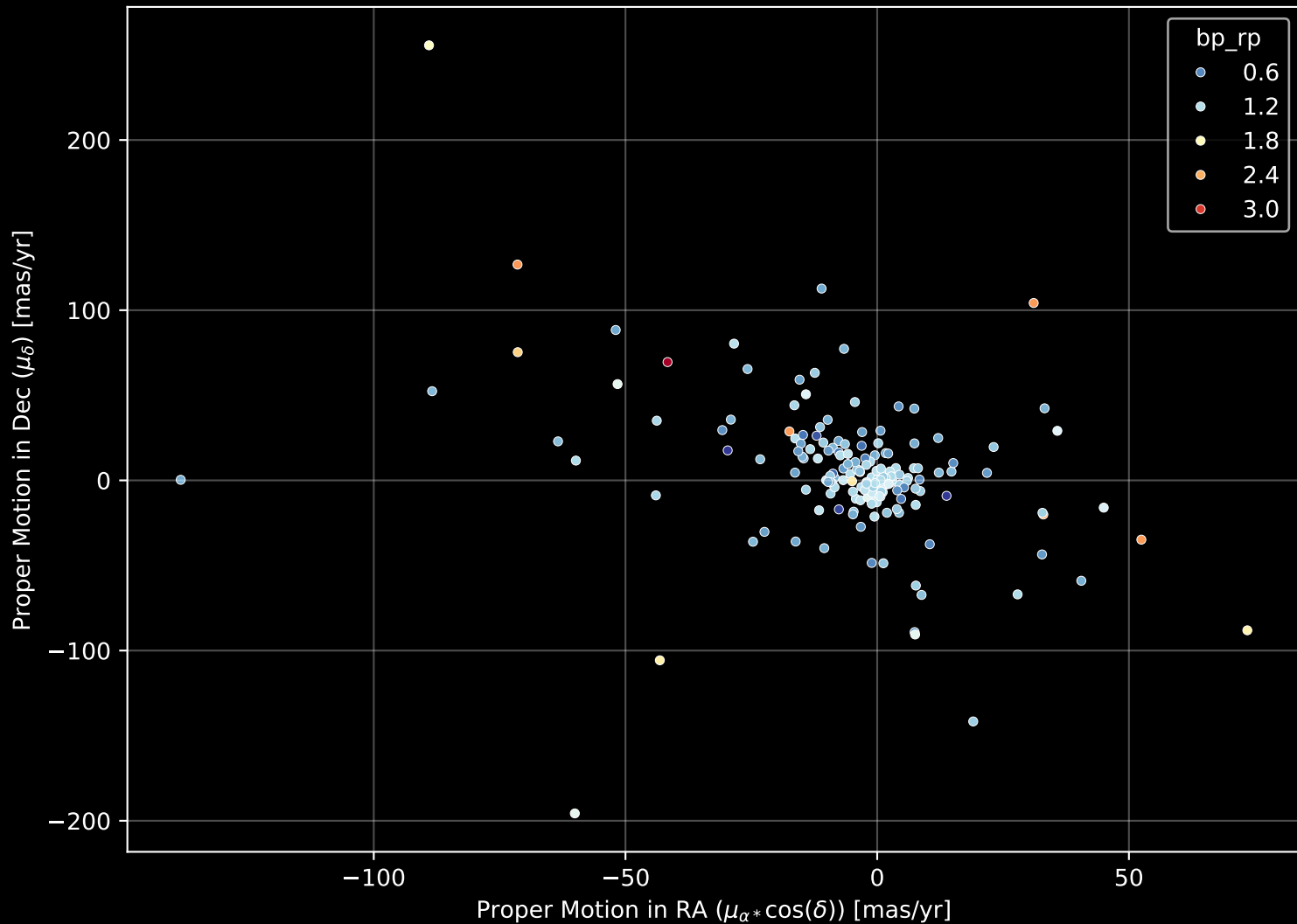
APOGEE DR17 Field: [CVZTILE_098+34_btx] Proper Motion Diagram (n= 176)
