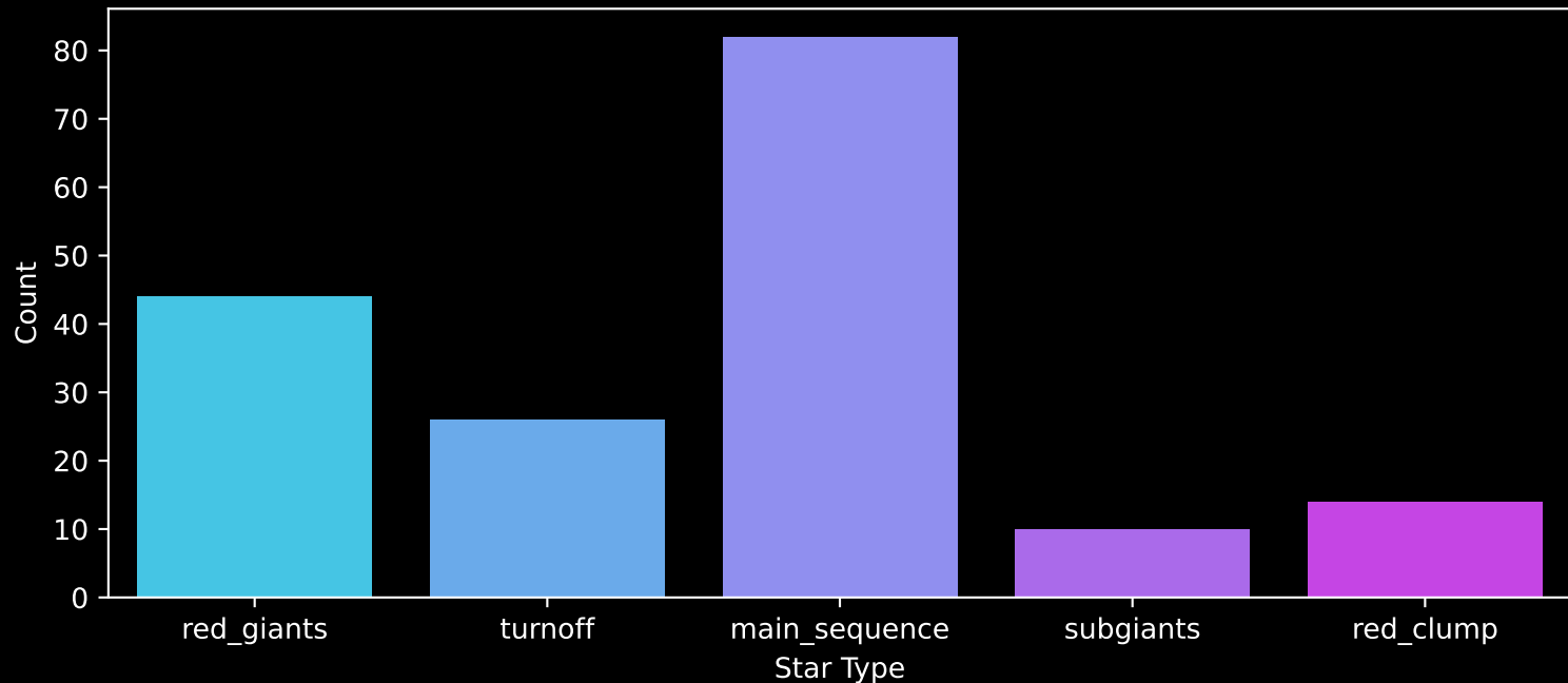
APOGEE DR17 Field: [CVZTILE_098+34_btx] Count plot of Star Type
