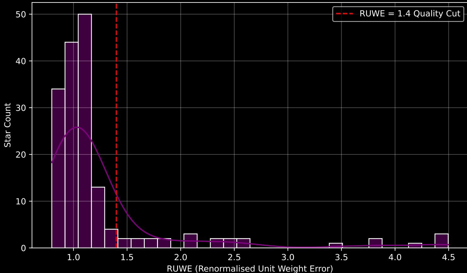
GAPOGEE DR17 Field [CVZTILE_098+34_btx] RUWE Distribution (n= 169)
