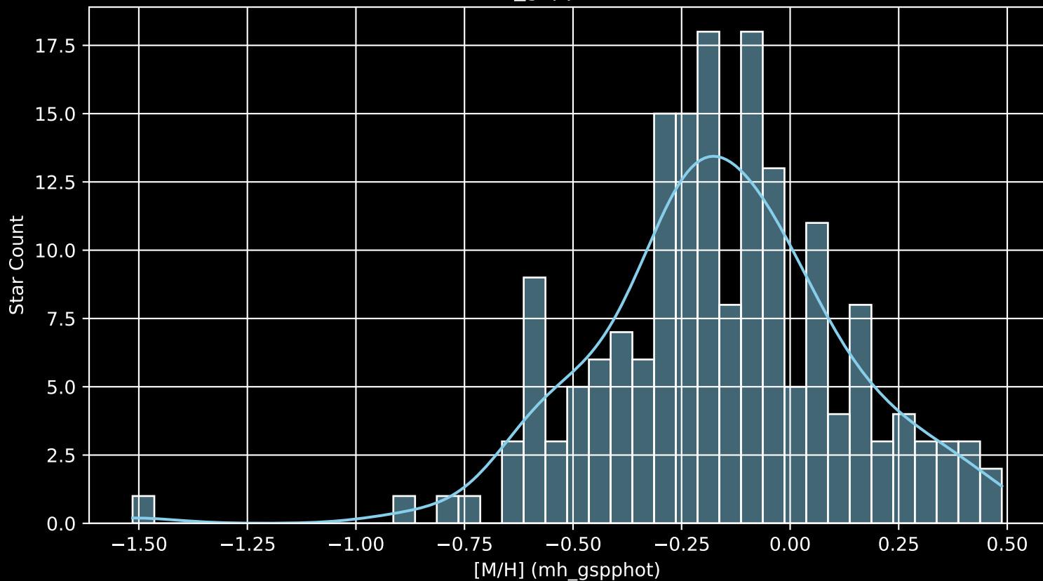
APOGEE DR17 Field: [CVZTILE_098+34_btx [M/H] (mh_gspphot) (n= 176)
